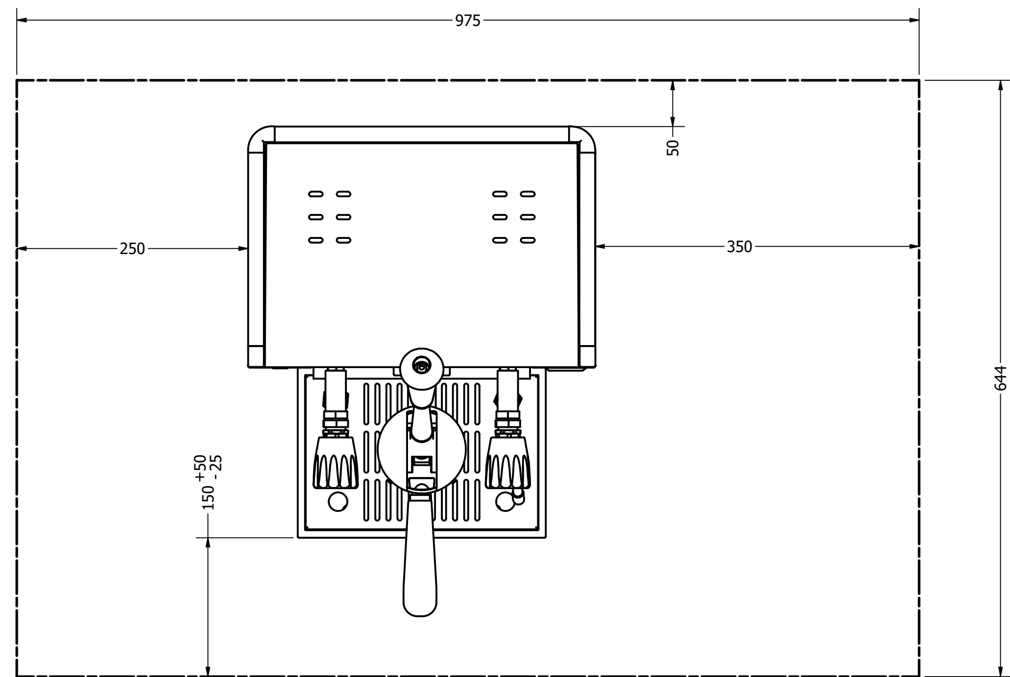
Suggested minimum clearances assuming a grinder placed to the right of the machine.
